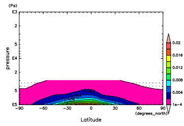
Figure 724: q at Feb. by DCPAM
