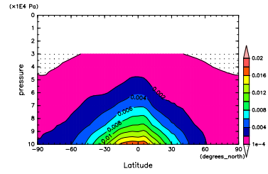
Figure 430: q at Dec. by DCPAM
