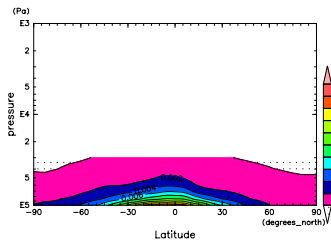
Figure 721: q at Jan. by DCPAM
