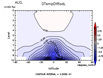
Figure 523: (\partial T/\partial t)_{LW} at Jul. by DCPAM by Figure 524: (\partial T/\partial t)_{LW} at Aug. by DCPAM
