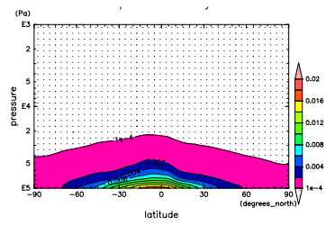
Figure 725: q at Feb. by NCEP
