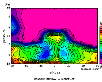
Figure 770: RH at May by NCEP
