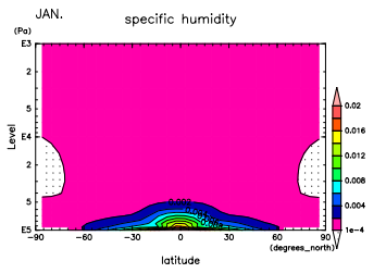
Figure 721: q at Jan. by DCPAM
