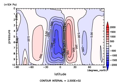
Figure 353: MSF at Oct. by NCEP
