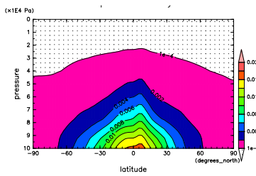
Figure 428: q at Nov. by NCEP
