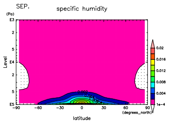
Figure 745: q at Sep. by DCPAM
