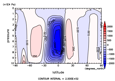
Figure 350: MSF at Sep. by NCEP
