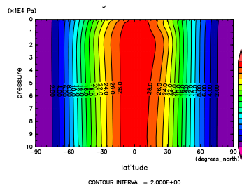
Figure 257: ANGMOM at Feb. by NCEP
