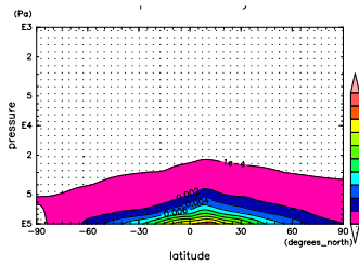
Figure 746: q at Sep. by NCEP
