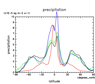
Figure 107: Rain at Nov. by DCPAM (red), NCEP (green), ECMWF (blue), and GPCP (black)
