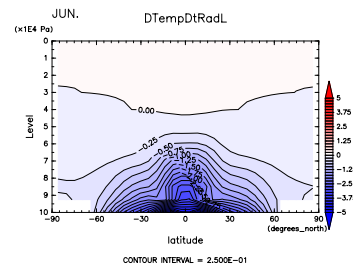
Figure 522: (\partial T / \partial t)_{LW} at Jun. by DCPAM
