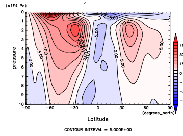
Figure 232: U at Jun. by DCPAM
