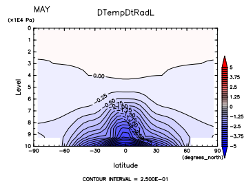
Figure 521: (\partial T / \partial t)_{LW} at May by DCPAM
