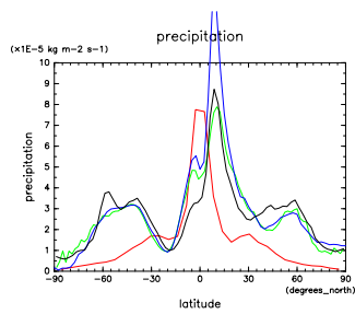
Figure 104: Rain at Aug. by DCPAM (red), NCEP (green), ECMWF (blue), and GPCP (black)
