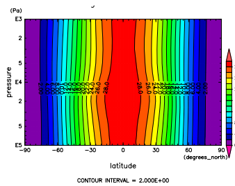
Figure 608: ANG MOM at Nov. by NCEP by Figure 611: ANG MOM at Dec. by NCEP
