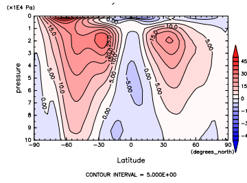
Figure 229: U at May by DCPAM
