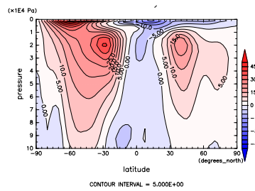
Figure 233: U at Jun. by NCEP
