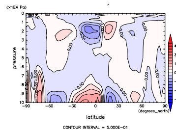
Figure 317: V at Oct. by NCEP
