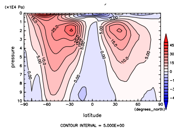
Figure 230: U at May by NCEP
