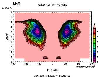
Figure 439: RH at Mar. by DCPAM
