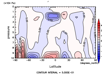
Figure 316: V at Oct. by DCPAM
