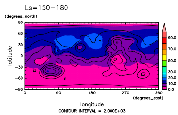
Figure 346: Prec. water at 14 LST and Ls=120^{\circ} - 150^{\circ} by DCPAM
