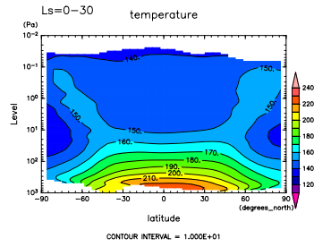
Figure 136: Temp at L_s=0^\circ-30^\circ by DCPAM
