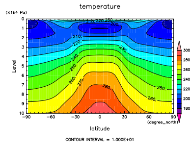
Figure 4: Temperature
