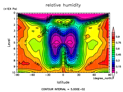
Figure 6: Relative humidity
