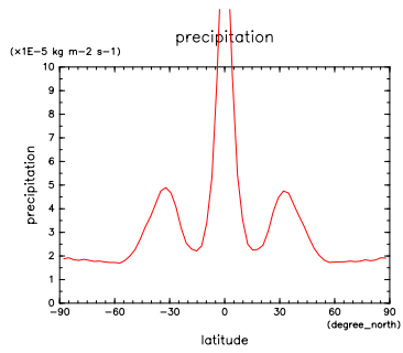
Figure 1: PRCP
