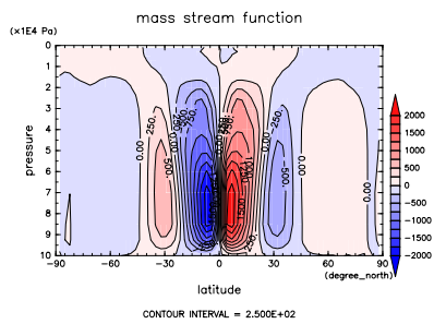
Figure 3: Mass stream function
