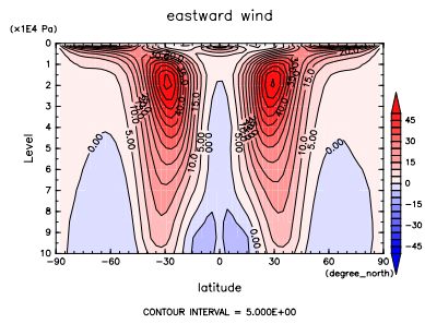
Figure 2: U
