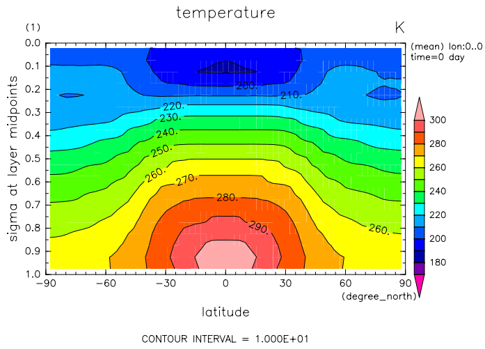
Figure 2: Zonal mean temperature by DCPAM
