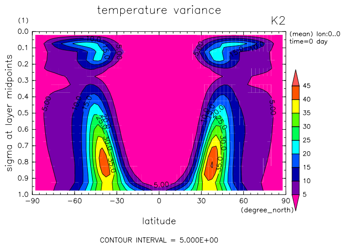
Figure 3: Zonal mean zonal eddy temperature squared by DCPAM
