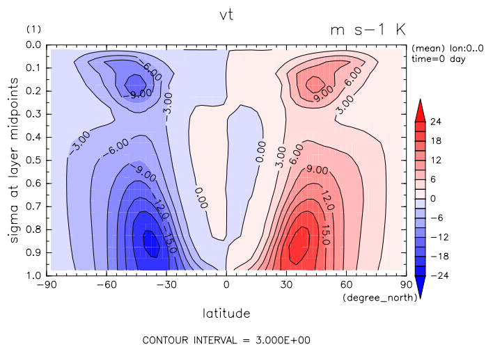
Figure 4: Zonal mean meridional wind and temperature covariance by DCPAM
