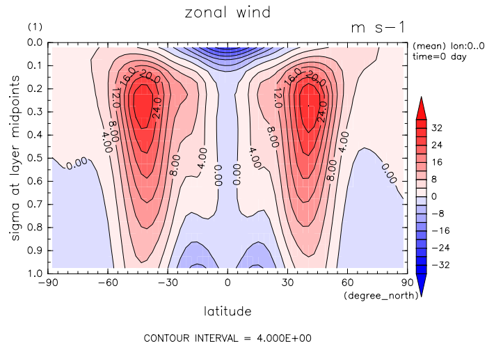
Figure 1: Zonal mean zonal wind by DCPAM
