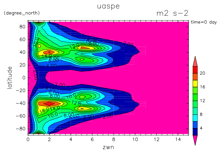
Figure 5: Spectrum of zonal wind by DCPAM
