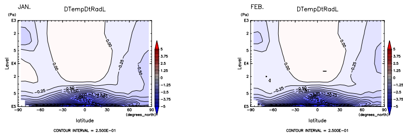
Figure 841: (\partial T/\partial t)_{LW} at Jan. by DCPAM Figure 842: (\partial T/\partial t)_{LW} at Feb. by DCPAM
