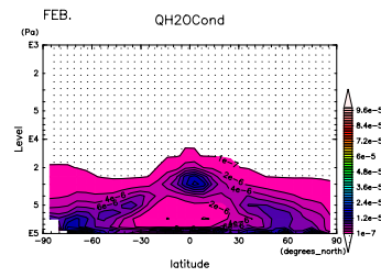
Figure 817: q_l + q_i at Jan. by DCPAM Figure 818: q_l + q_i at Feb. by DCPAM
