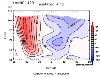
Figure 67: U at L_S=90^\circ-120^\circ by DC-PAM
